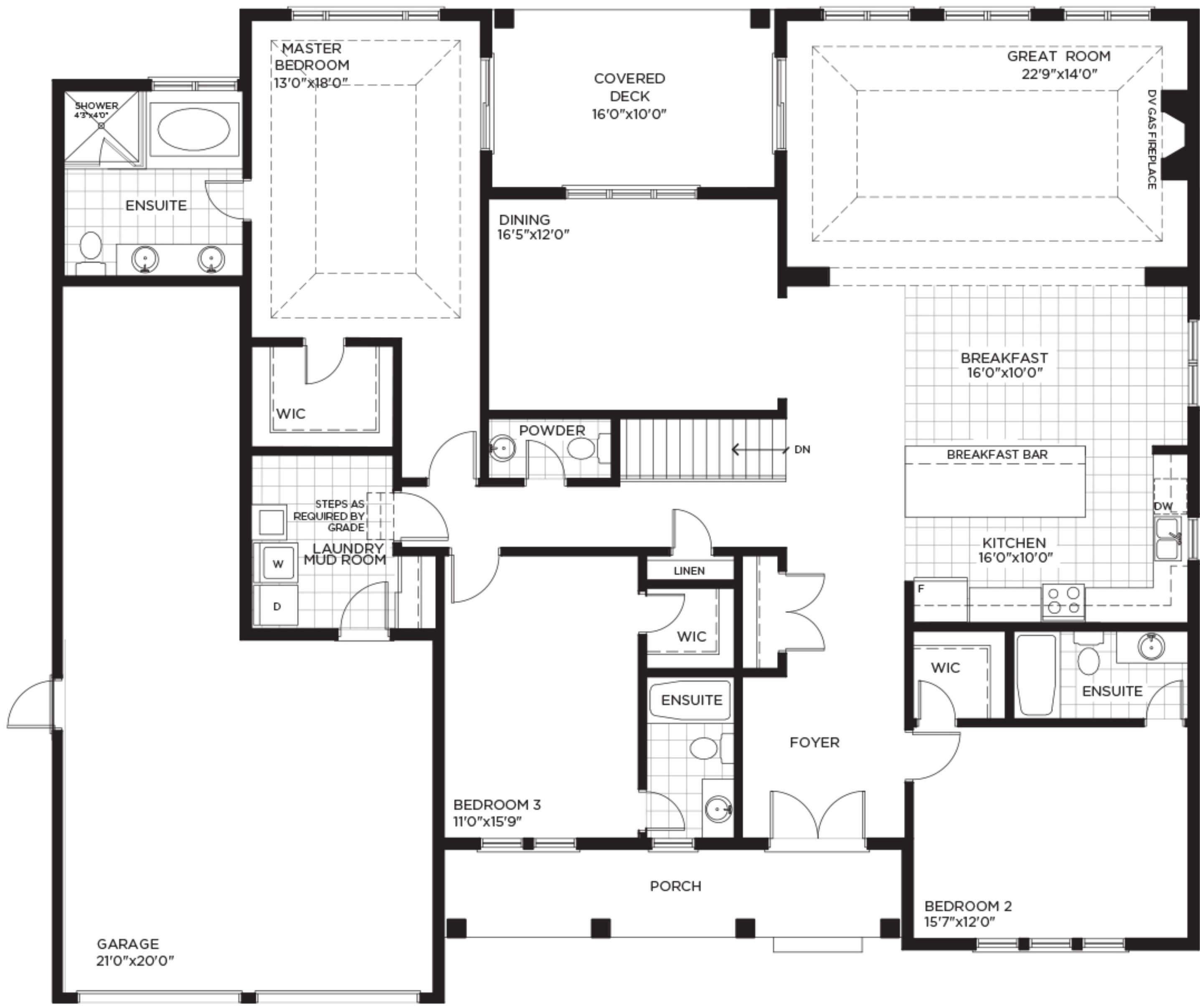
FIRST FLOOR PLAN ELEV. A
