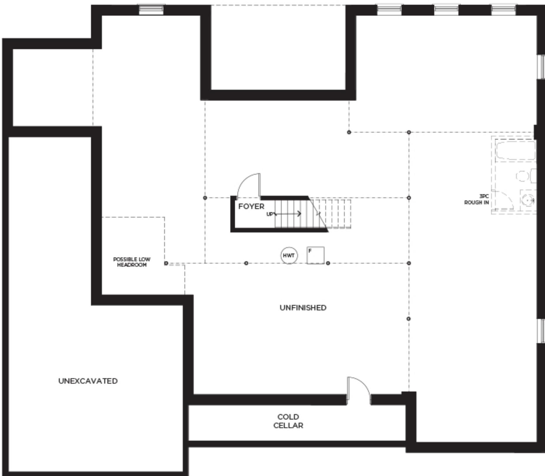
BASEMENT PLAN
