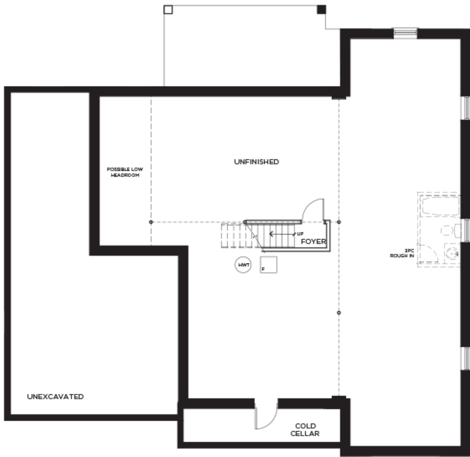
BASEMENT PLAN ELEV. A
