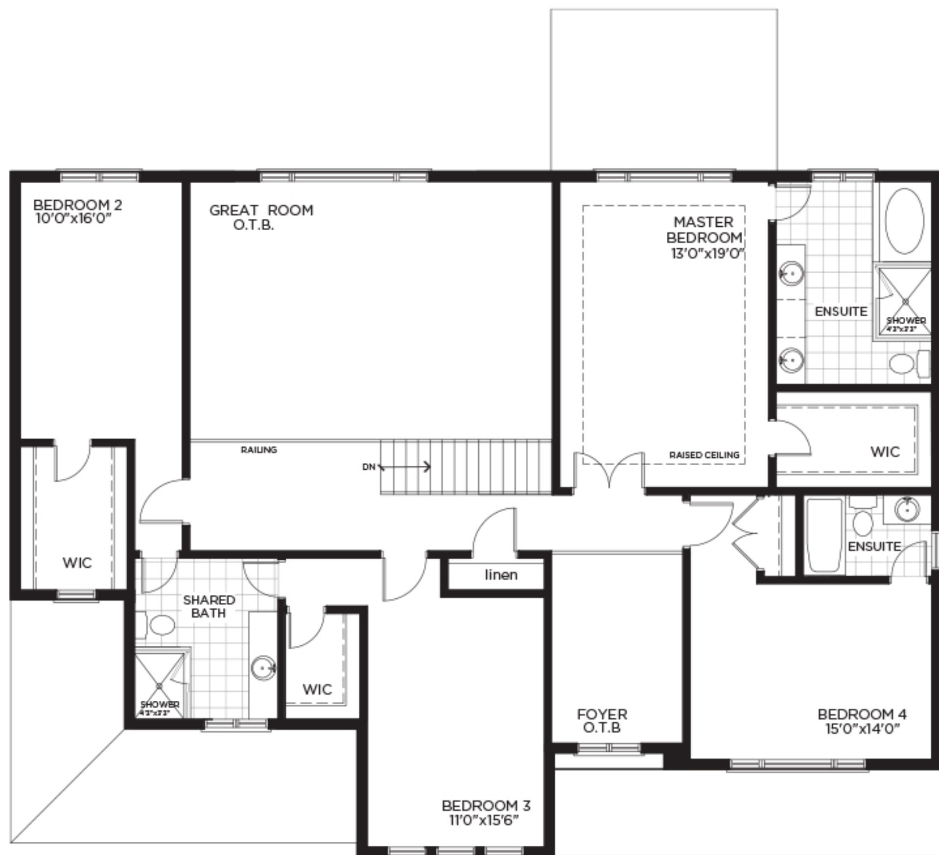
SECOND FLOOR PLAN ELEV. A
