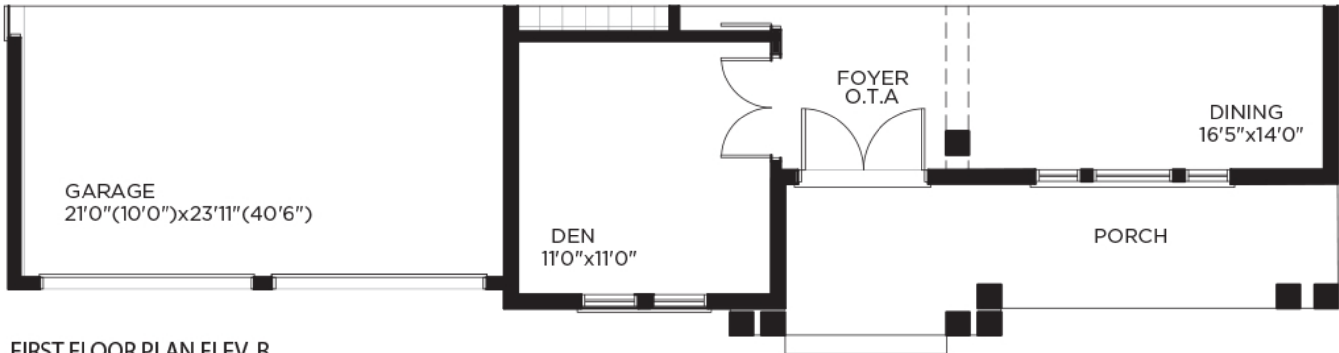
FIRST FLOOR PLAN ELEV. B
